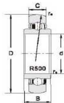
LR2...RRU
