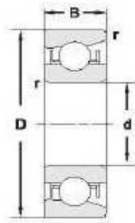
Open type
